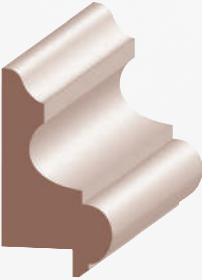
1-3/16 x 2-3/16 Raised Panel Cap [with 3/4" Rab't] 611P Poplar N
